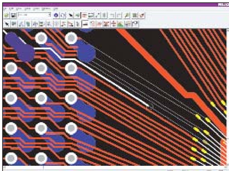
PADS Router, our interactive route editor, supports any-angle routing to substrate pads, with or without a netlist
